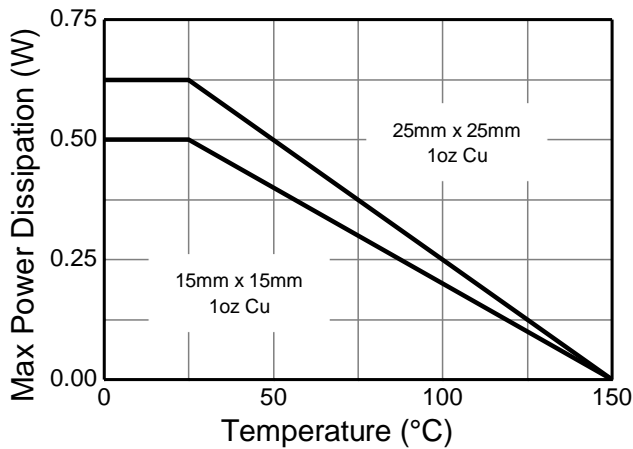
Derating Curve
